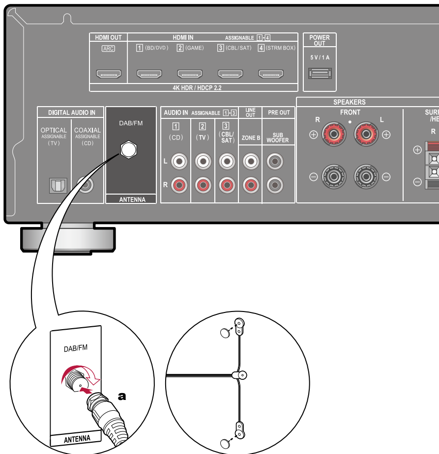
a Antenne DAB/FM
