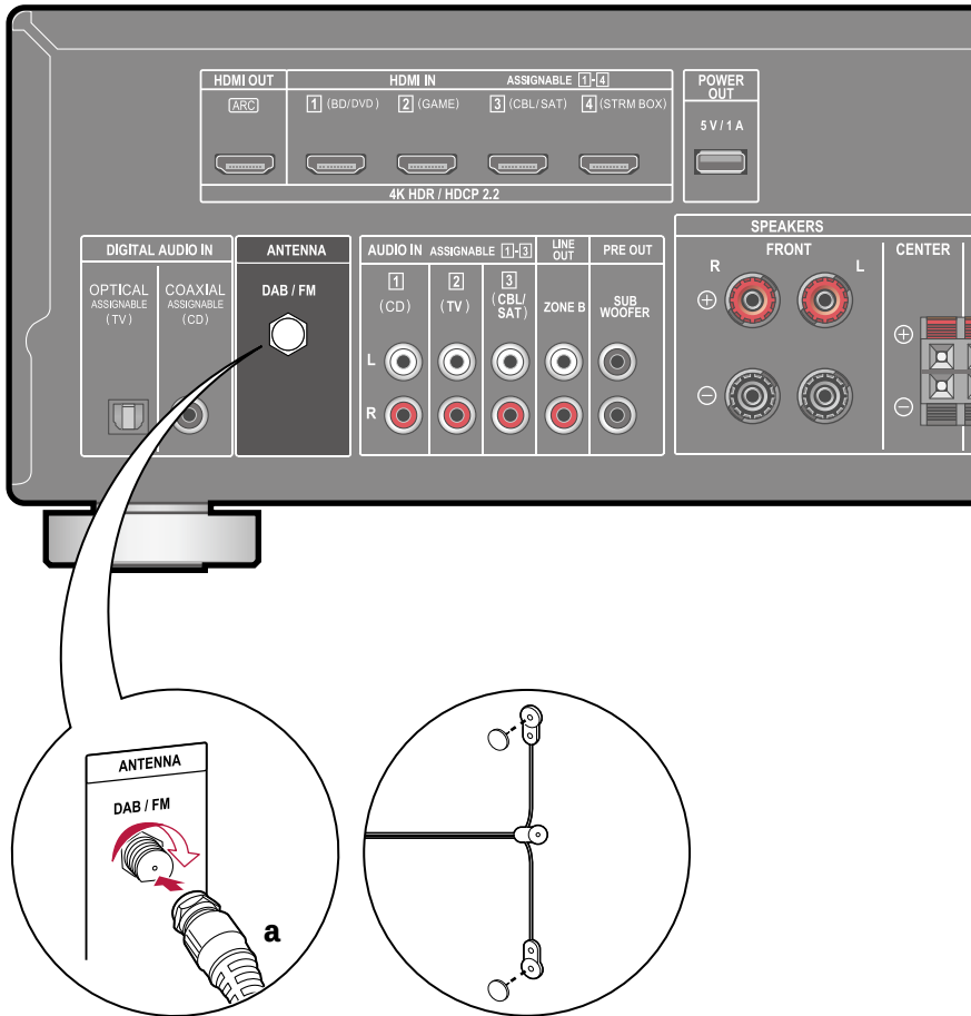
a DAB/FM-antenne
